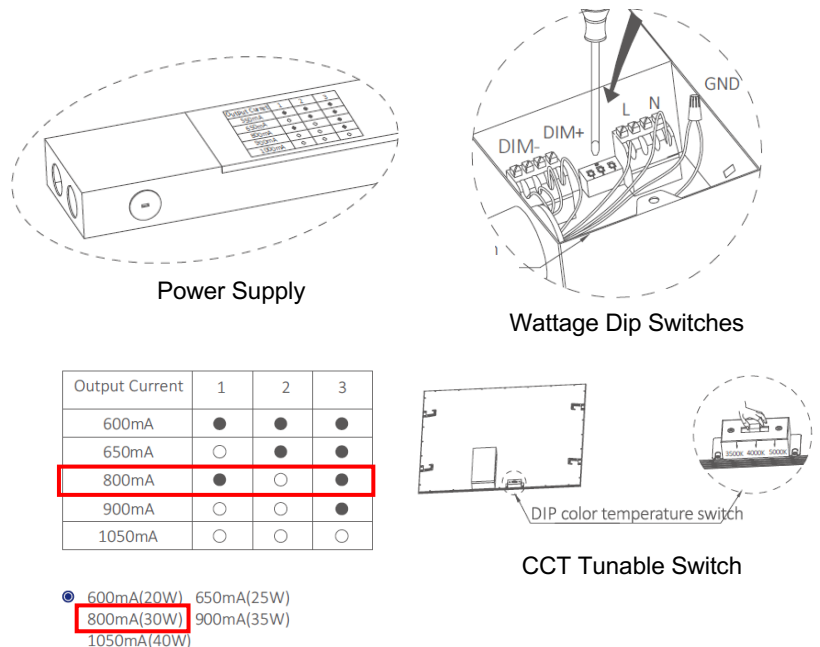
Wattage Dip Switch Settings
